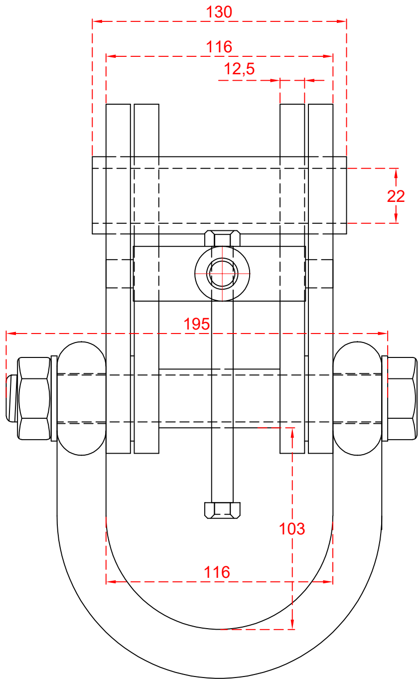
S3X Fixed Jaw Girderclamp Assembly 5080kgs (5T) WLL 76 - 190mm Adjustment 10kg Average Weight
